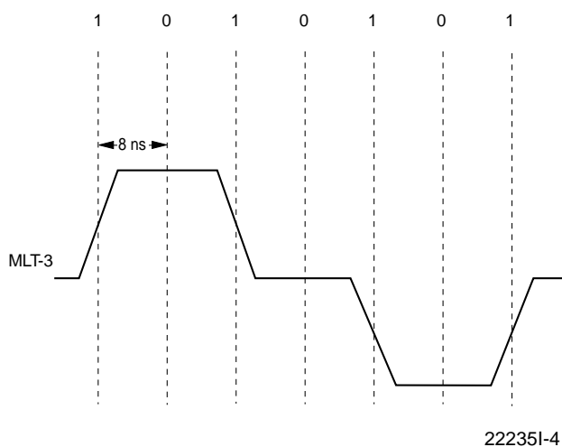
Figure 2. MLT-3 Waveform
